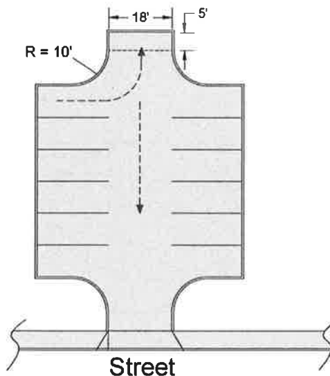
Figure 17.75.04 Parking Lot Minimum Turnaround Standard
